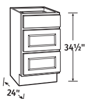
Drawer Base
